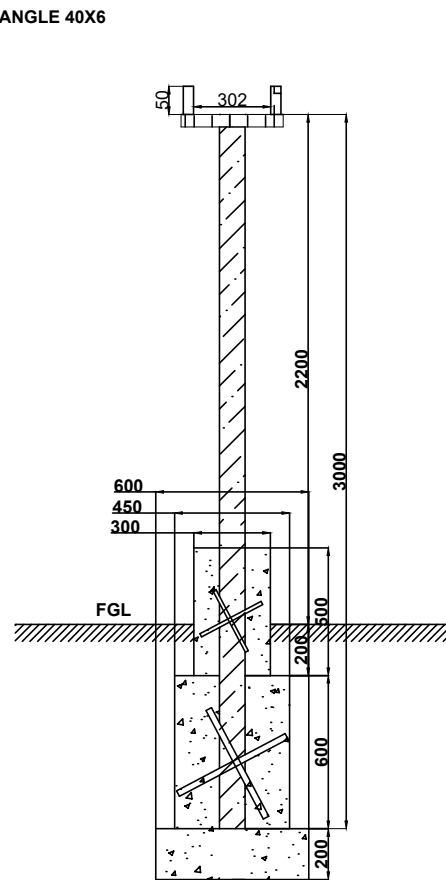
CIVIL FOUNDATION
