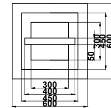
CIVIL FOUNDATION (TOP VIEW)
