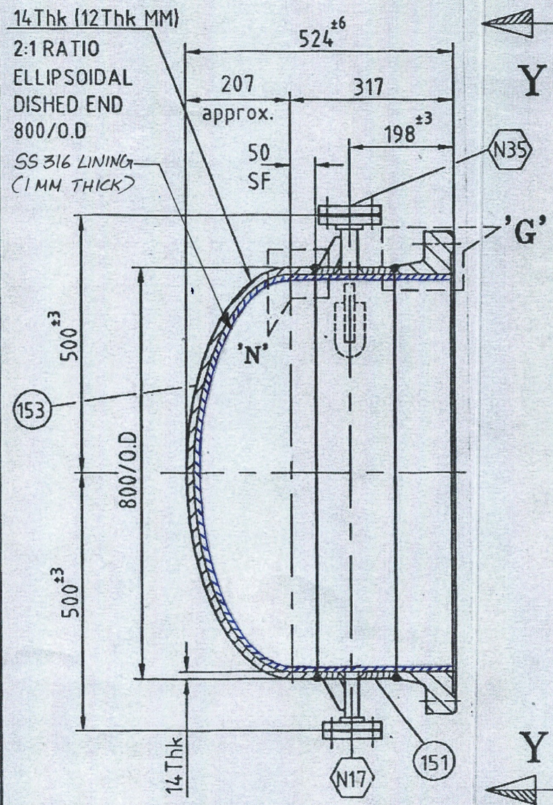
DETAIL OF COVER SHELL ASSEMBLY END VIEW - YY
