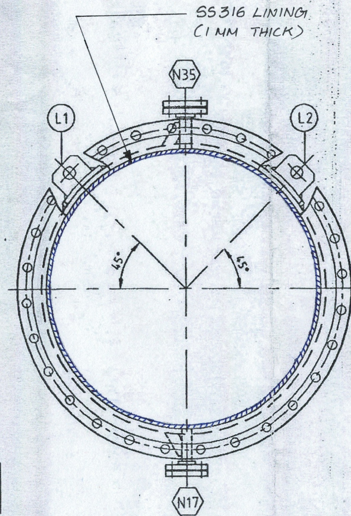
DETAIL OF COVER SHELL ASSEMBLY END VIEW - YY
